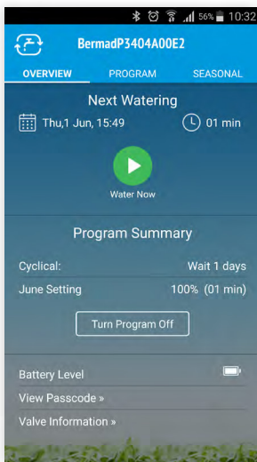
Overview Screen
